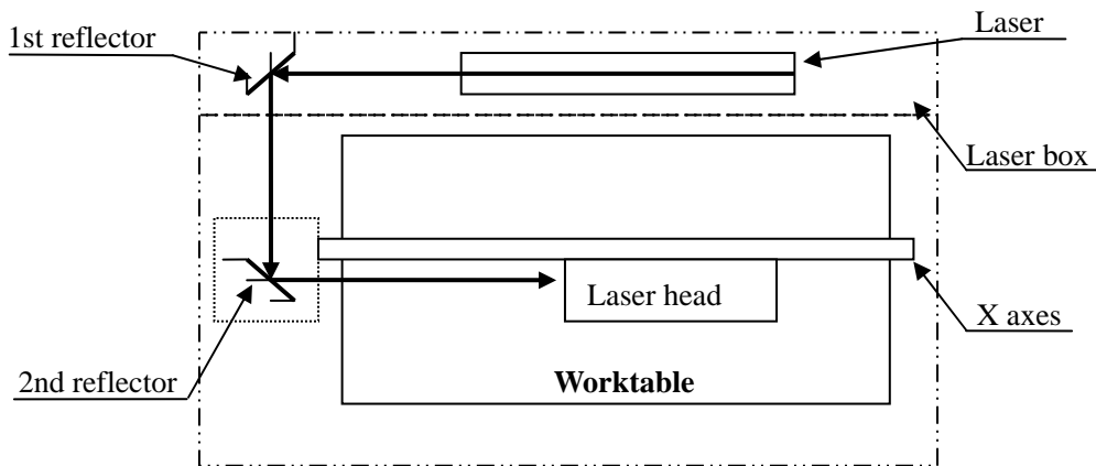
Pic.2-8 Optical path
