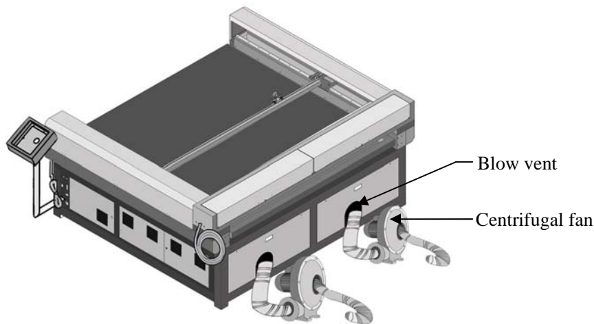
Pic2-5 Air exhaust system
