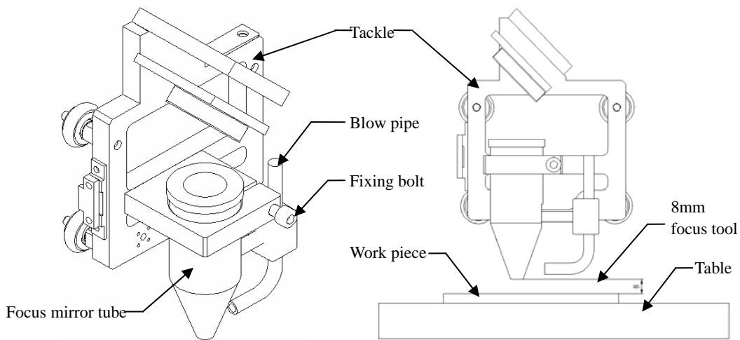
Pic. 2-10 Adjusting focus
