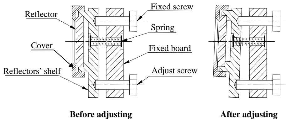
Pic.2-6 1st and 2nd reflector shelves
