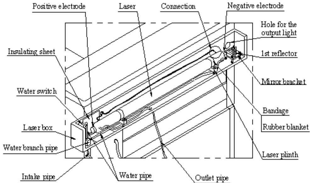
Pic.2-1 Laser system
