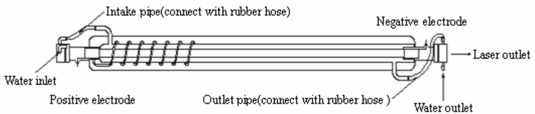
Pic.2-2 Glass laser tube
