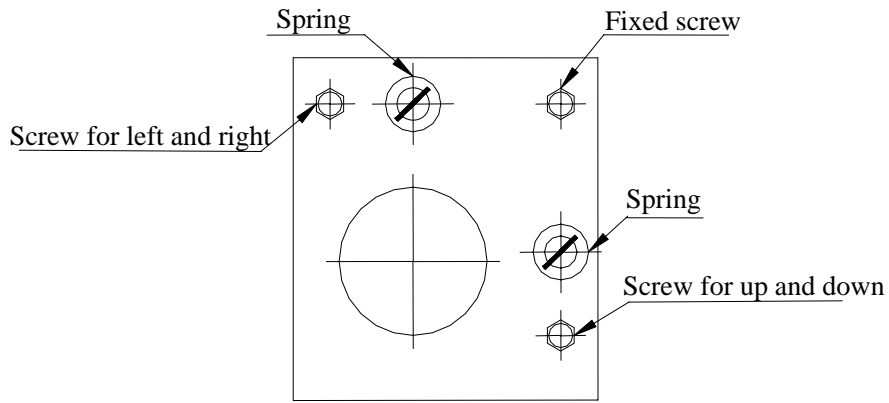
Pic.2-7 Adjust screw of the reflectors' shelf
