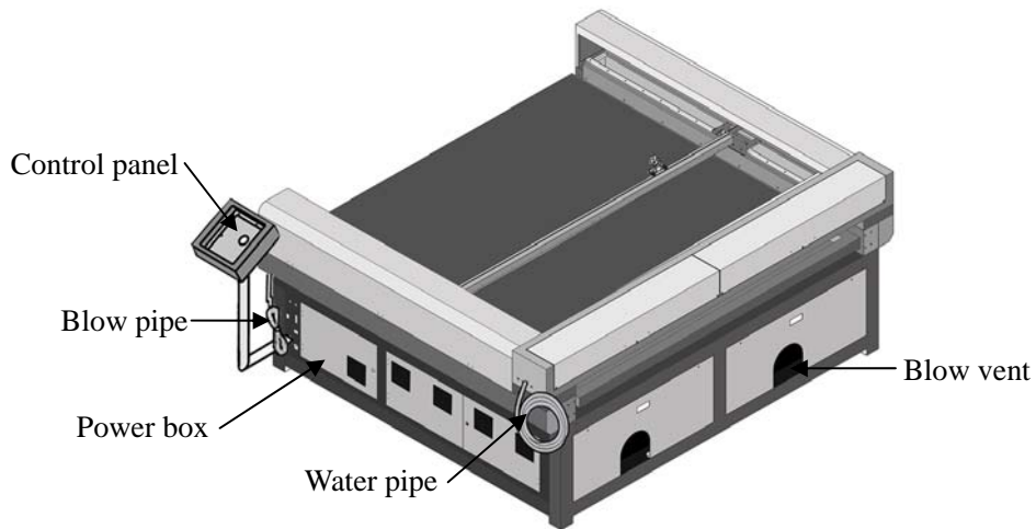
Pic.1-1 Left side of the machine
