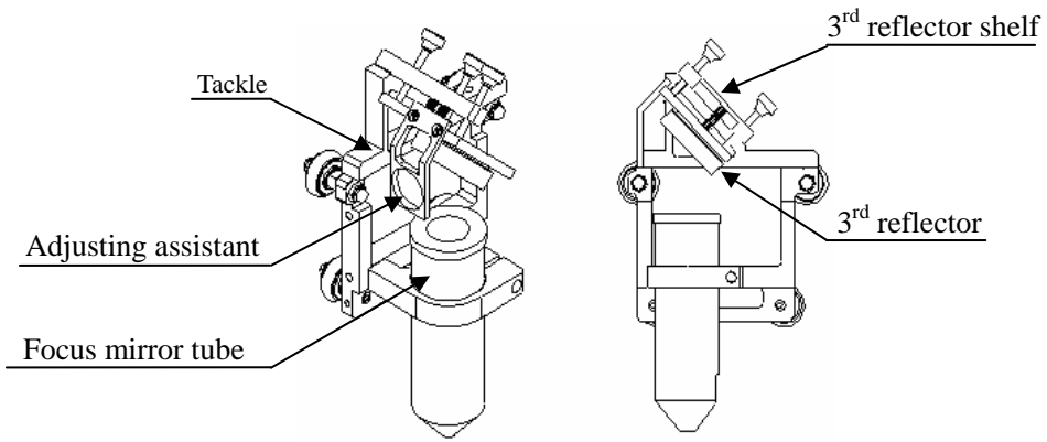
Pic.2-9 Laser head configuration
